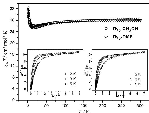
Figure 2. Temperature dependence of the \chi_M T value at 1000 Oe for \text{Dy}_2\text{-DMF} ( \nabla ) and \text{Dy}_2\text{-CH}_3\text{CN} ( \circ ). Inset: Plots of magnetization ( M ) versus applied field ( H ) at 2, 3, and 5 K for \text{Dy}_2\text{-CH}_3\text{CN} (left) and \text{Dy}_2\text{-DMF} (right). The solid lines correspond to calculated fits to the data.
